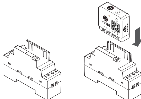
Roller Shutter Module SIN-2-RS-XX
